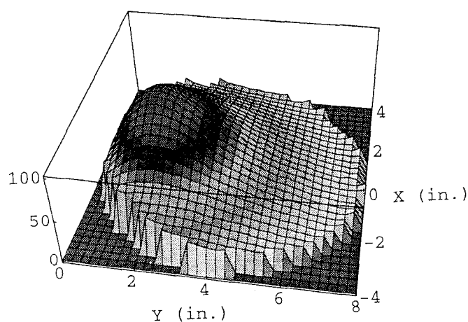
Fig. 2(a). Surface plot of the measured two dimensional thickness profile obtained from a 3" YBCO target on a stationary 8" Si wafer. The thickness is normalized on a scale of 0 to 100%.
